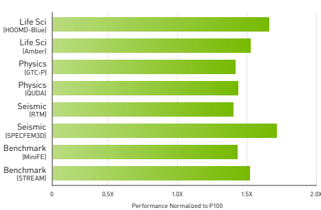
1.5X HPC Performance in One Year with NVIDIA Tesla V100
